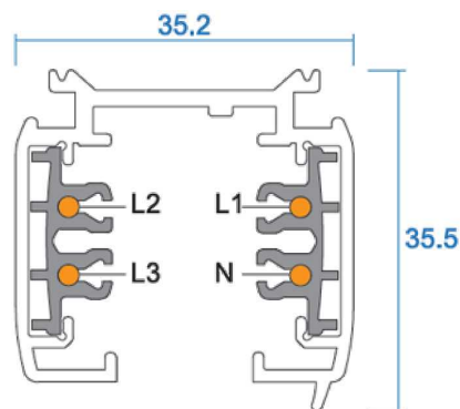
3 Circuits Track
