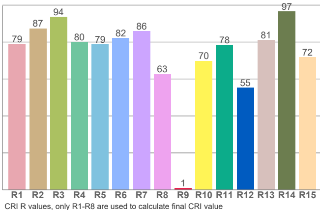
Colour Rendering Index per reference colour (CIE 1995)
